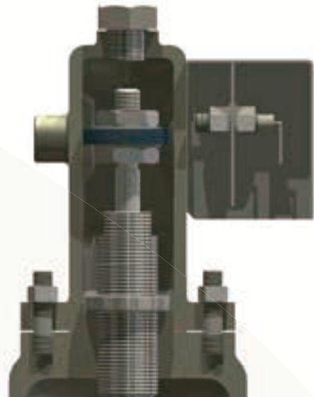
MAGNETIC SENSOR
