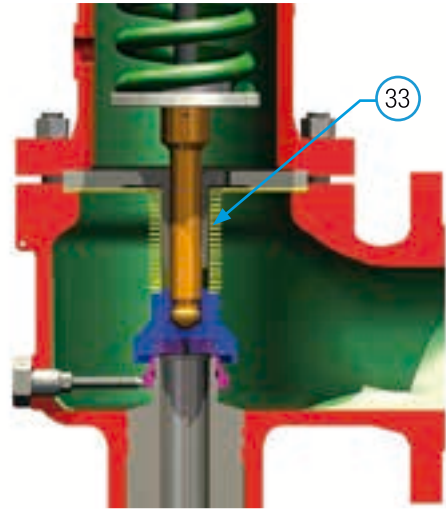
BELLOWS VALVE
